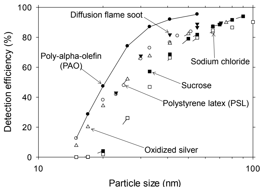
Figure B.1 — An example data set that presents the chemical composition dependence of the detection efficiency of a butanol-based CPC. Reprinted from [23] with permission from Elsevier.
