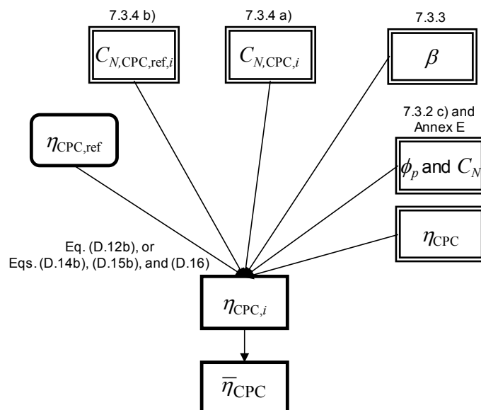
Figure 7 — A map of parameters and equations that are needed to derive the detection efficiency in calibration with a reference CPC. Plain rectangles represent calculated values while double-lined and round-cornered rectangles are for measured values and values taken from certificates, respectively
