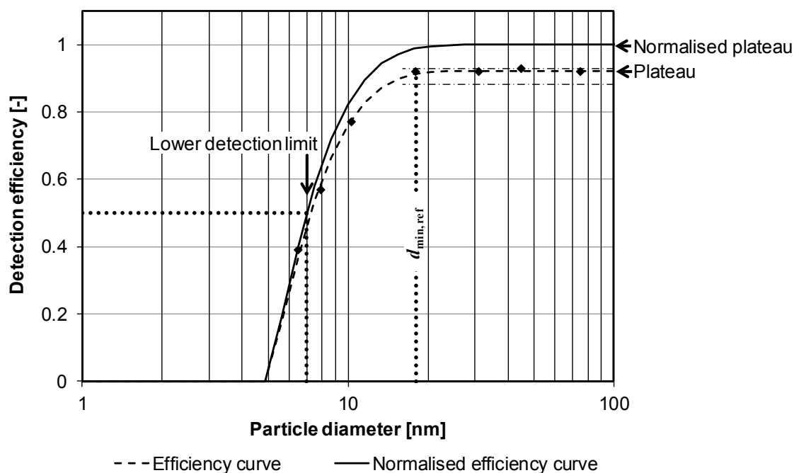
Figure A.2 — Particle size dependence of the detection efficiency of a reference CPC with particles of a given concentration and particle type
