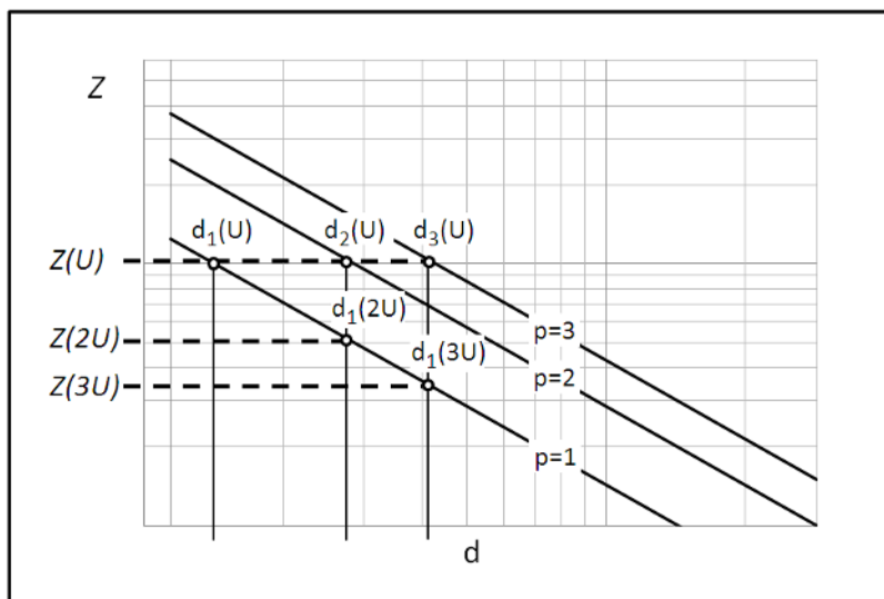
Figure E.1 — Relationship between mobility, DEMC-voltage and particle sizes
