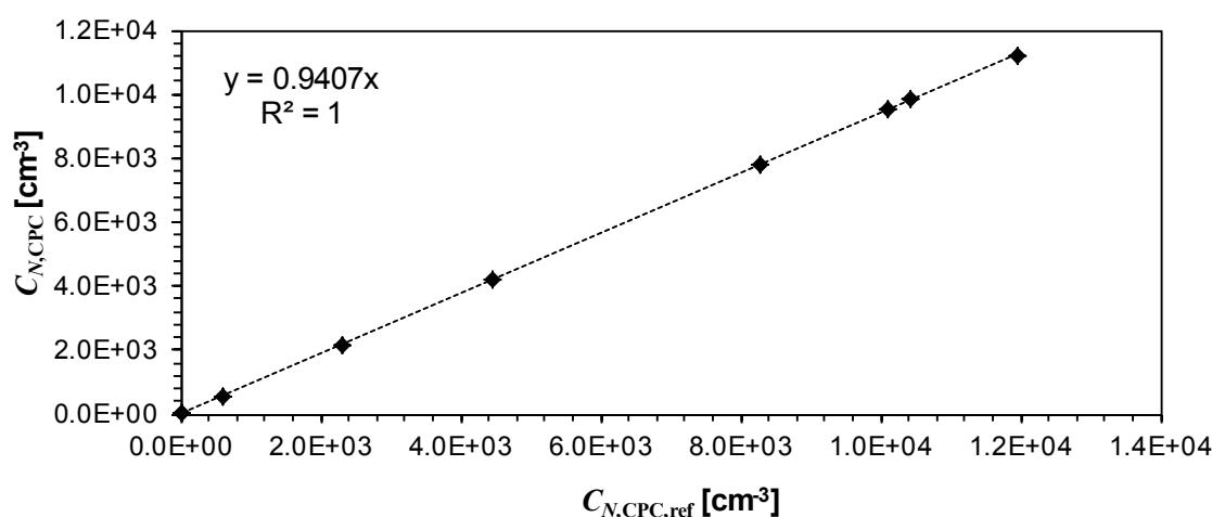
Figure A.5 — Simple linear regression plot between the test CPC and the reference instrument (data from Table A.1). The slope is 0,9407
