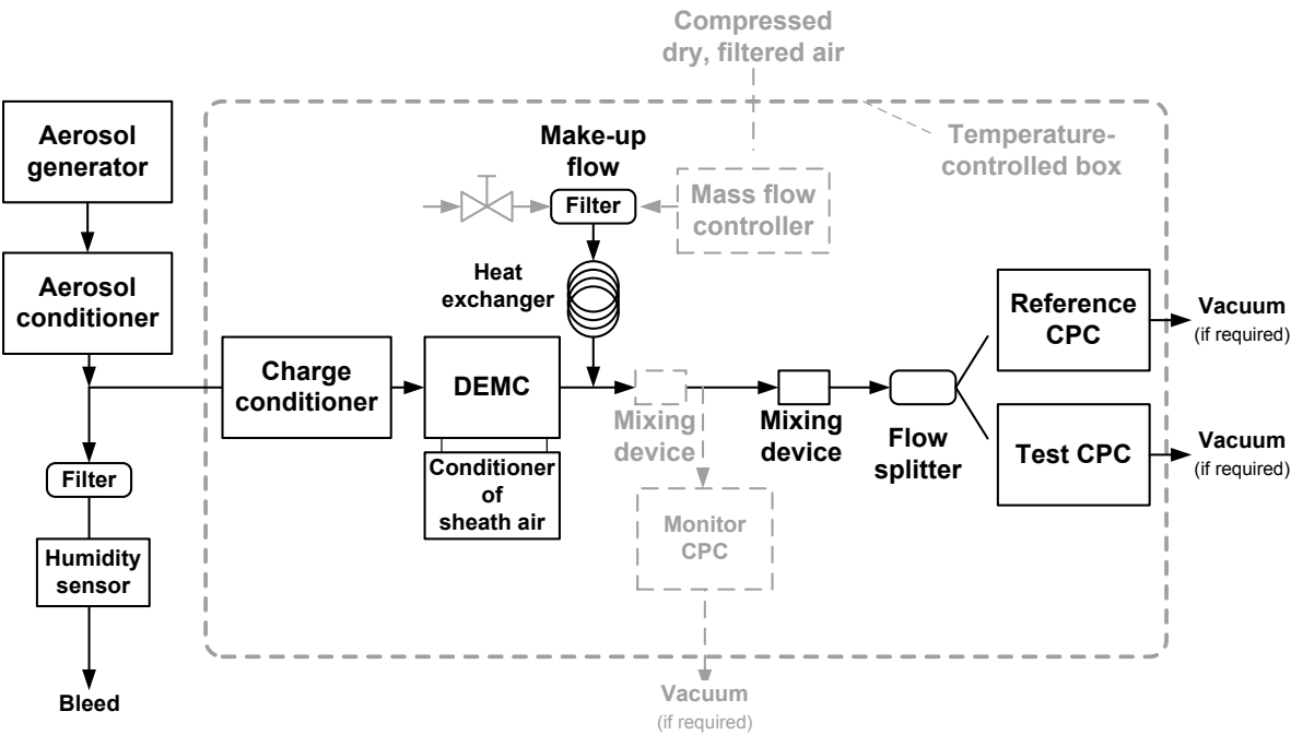
Figure 6 — The calibration setup with CPC as reference instrument. Dashed lines in grey show equipment that is not required, but highly recommended.
