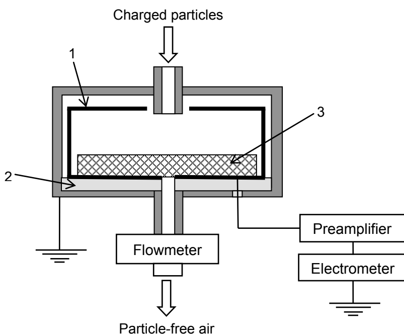
Figure 3 — Schematic diagram of an FCAE: (1) is a Faraday cup to collect electrical charge from charged collected particles and to reduce externally-induced electro-magnetic noise, (2) is a very-high-resistance electrical insulator to isolate the filter from electrical ground, and (3) is a high-efficiency particulate air (HEPA) filter to trap airborne charged particles. (Adapted from ISO 15900.)
