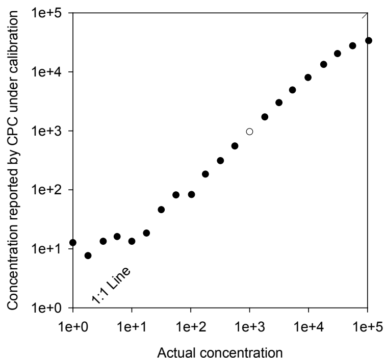
Figure A.1 — Relationship between the actual concentration and the concentration reported by a CPC in single particle counting mode illustrating false counts and coincidence losses with particles of a given size and type
