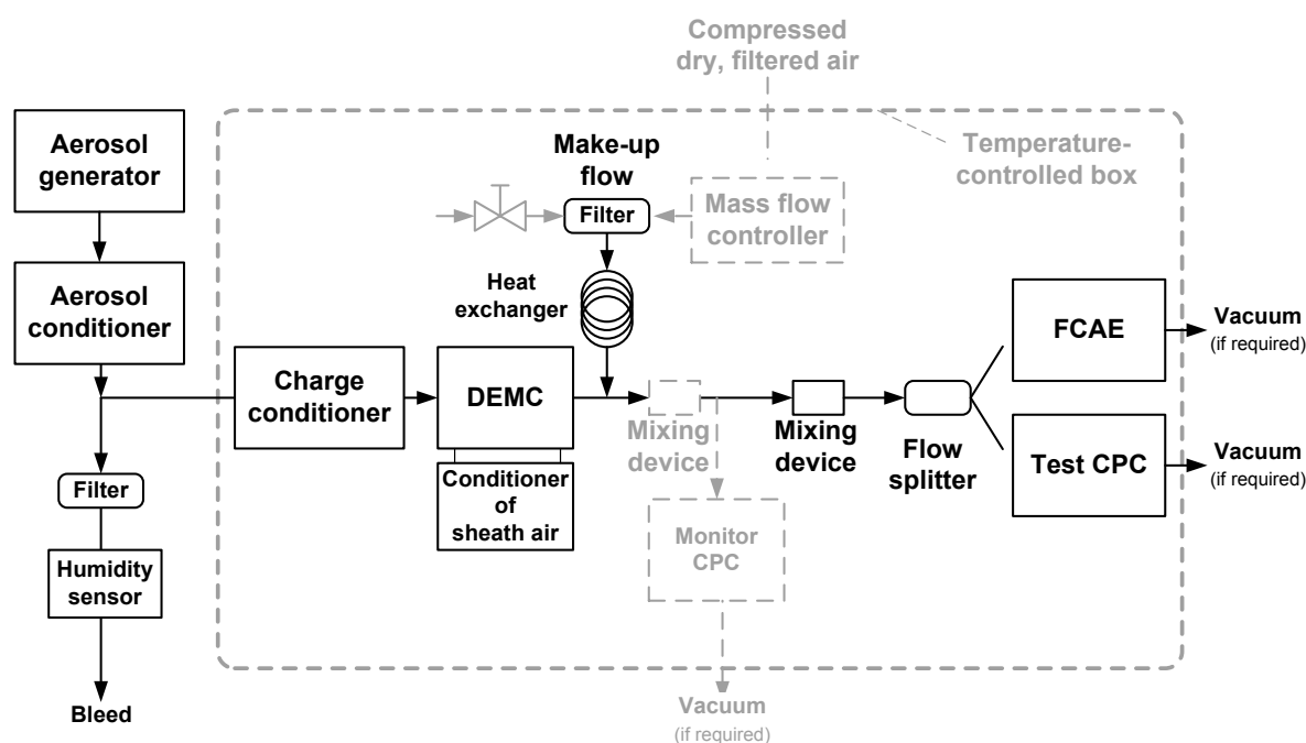
Figure 4 — The calibration setup with FCAE as reference instrument. Dashed lines in grey show equipment that is not required, but highly recommended.
