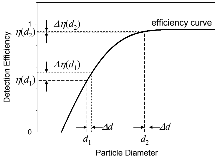
Figure N.1 — Errors in the CPC detection efficiency due to errors in particle size and their dependence on the slope of the efficiency curve
