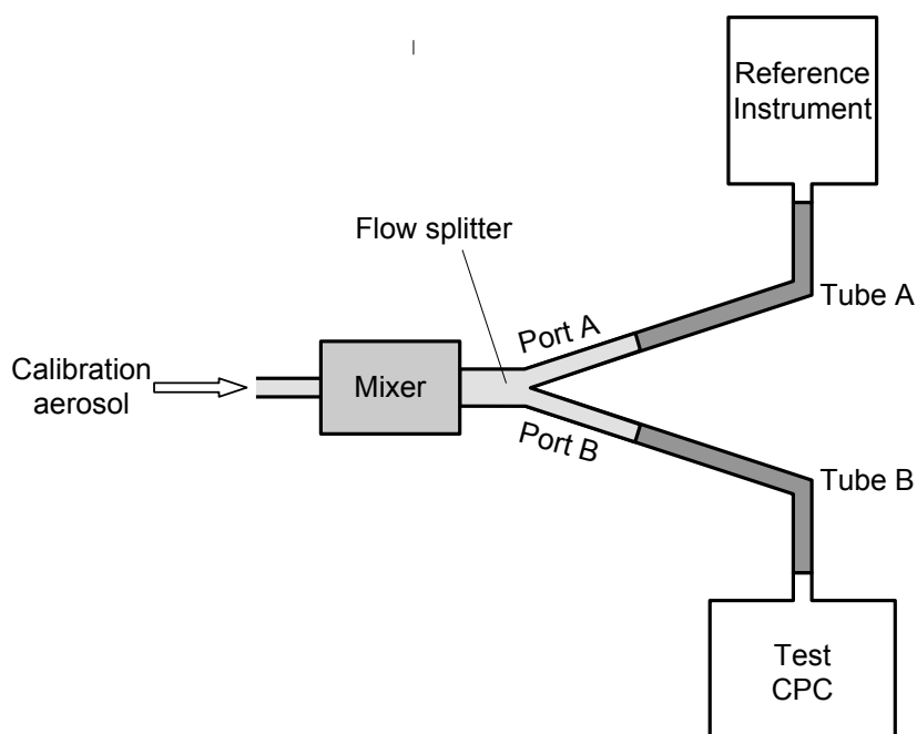
Figure H.1 — The first connection configuration of the flow splitter and the tubes after it
