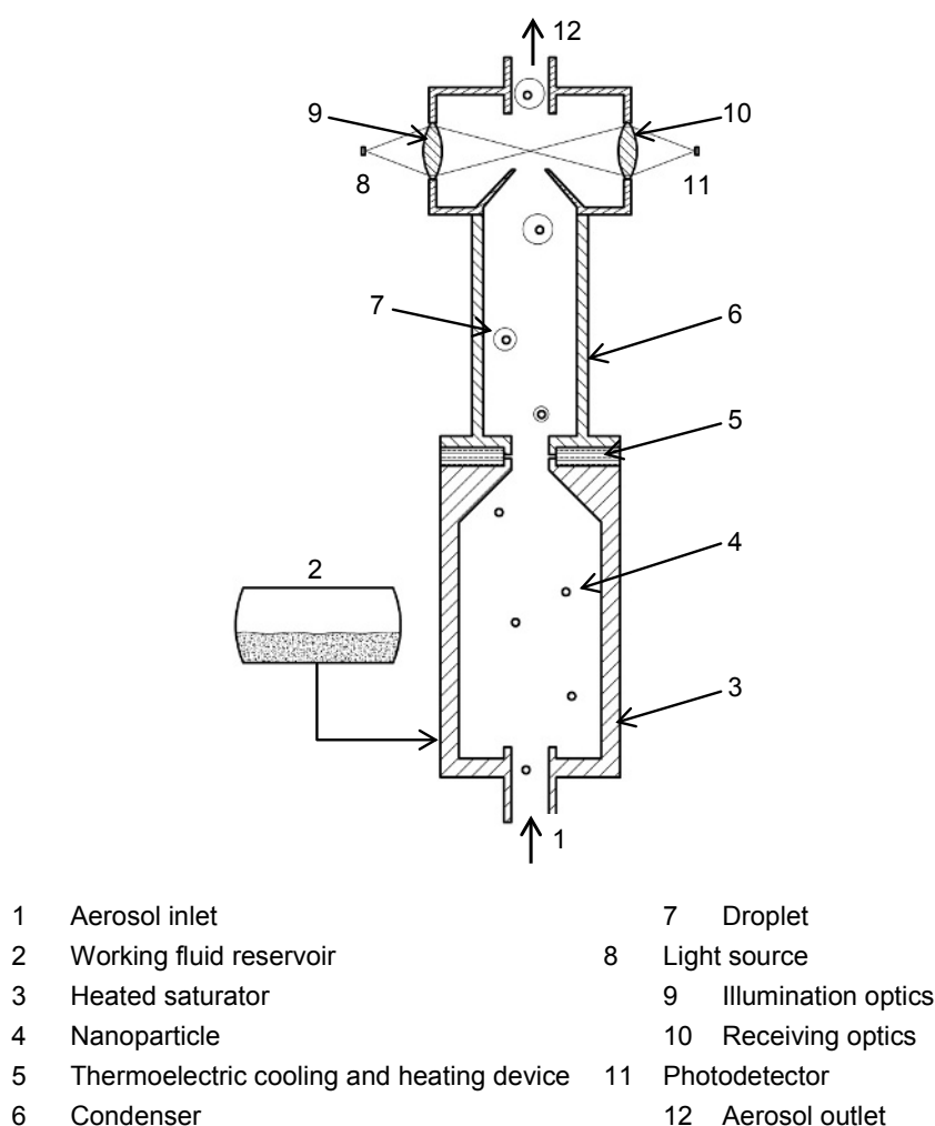
Figure 1 — Principle of a laminar flow CPC
