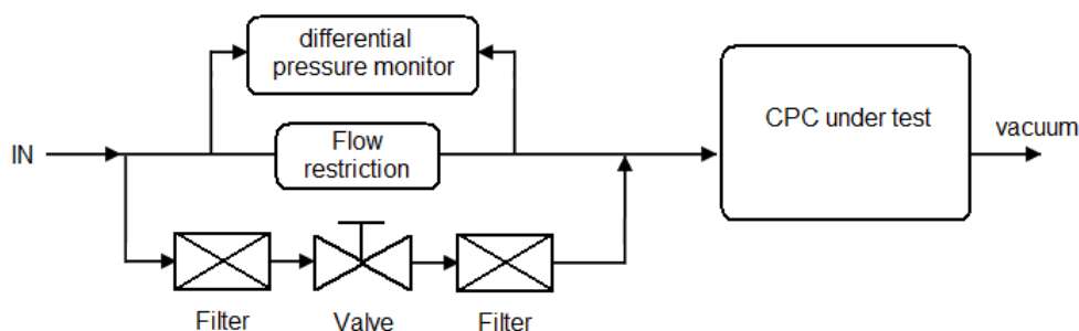
Figure I.1 — Schematic of the recommended diluter and CPC configuration
