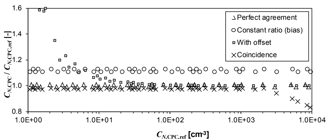
Figure A.4 — Typical patterns of residual plots with good precision
