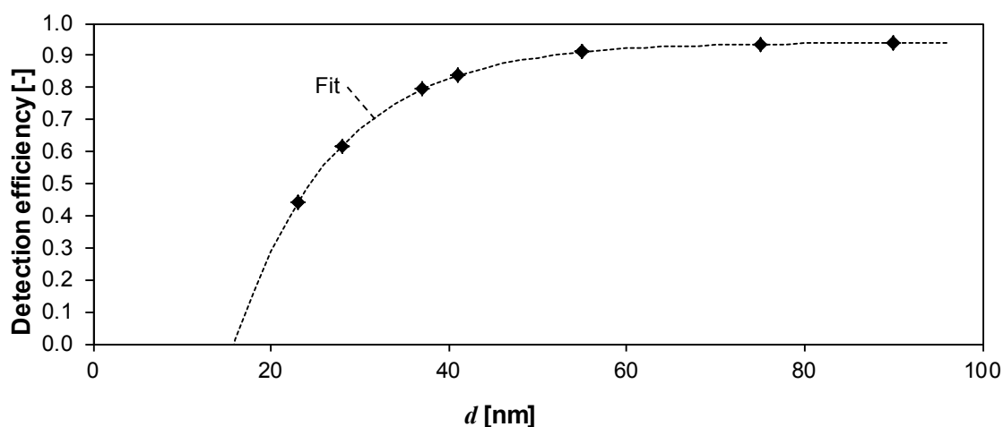
Figure A.7 — Fitted detection efficiency curve of the test CPC as a function of the size
