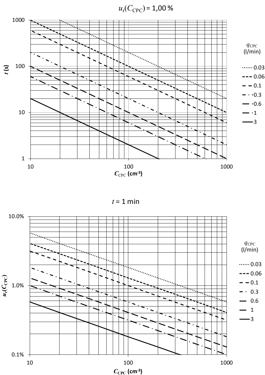
Figure O.1 — Diagrams that illustrate the relationship of the O.counting uncertainty with the CPC detector flow rate and averaging time
