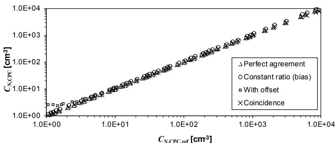
Figure A.6 — Typical patterns of non-ideal behaviour of CPCs (see Figure A.4 and discussion there)
