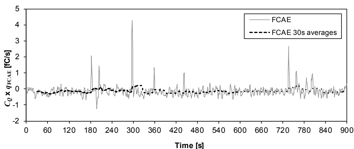
Figure J.2 — Zero levels of the FCAE
