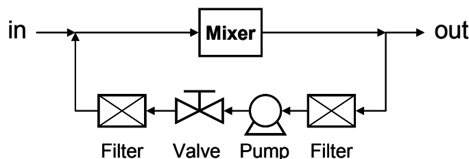
Figure G.2 — Schematic of the dilution loop
