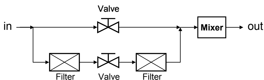
Figure G.1 — Schematic of the dilution bridge
