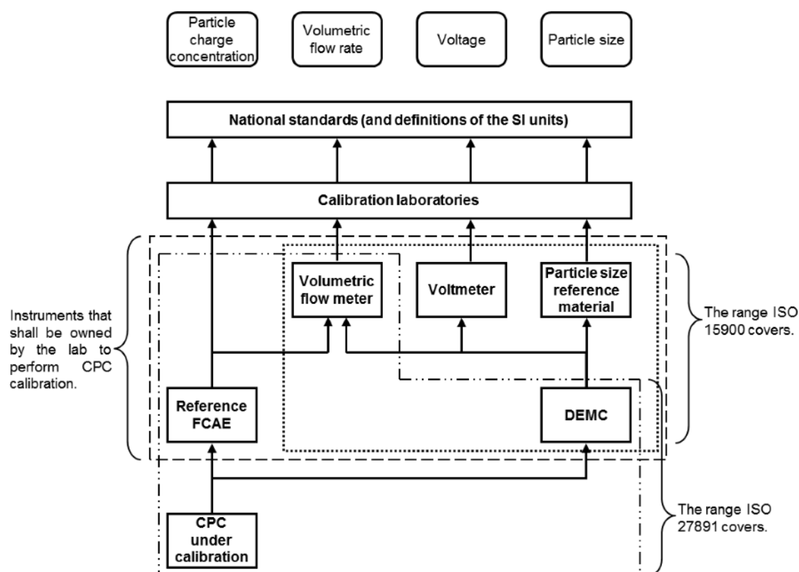
Figure F.1 — Traceability diagram for calibration with an FCAE
