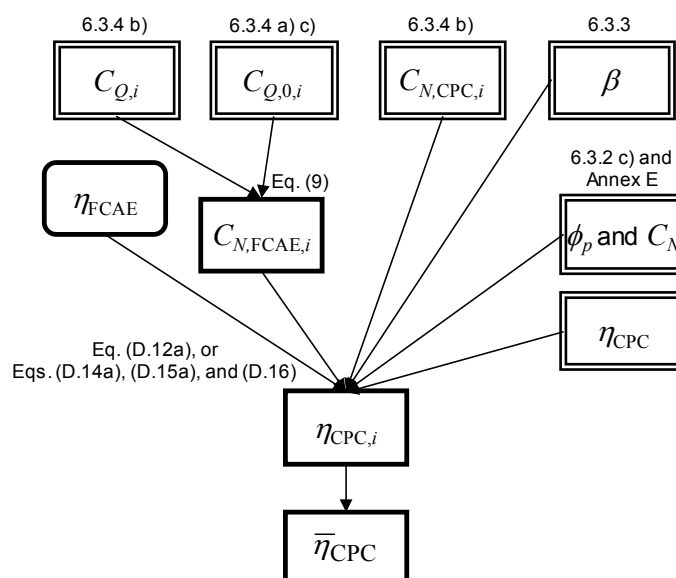
Figure 5 — A map of parameters and equations that are needed to derive the detection efficiency in calibration with an FCAE. Plain rectangles represent calculated values while double-lined and round-cornered rectangles are for measured values and values taken from certificates, respectively
