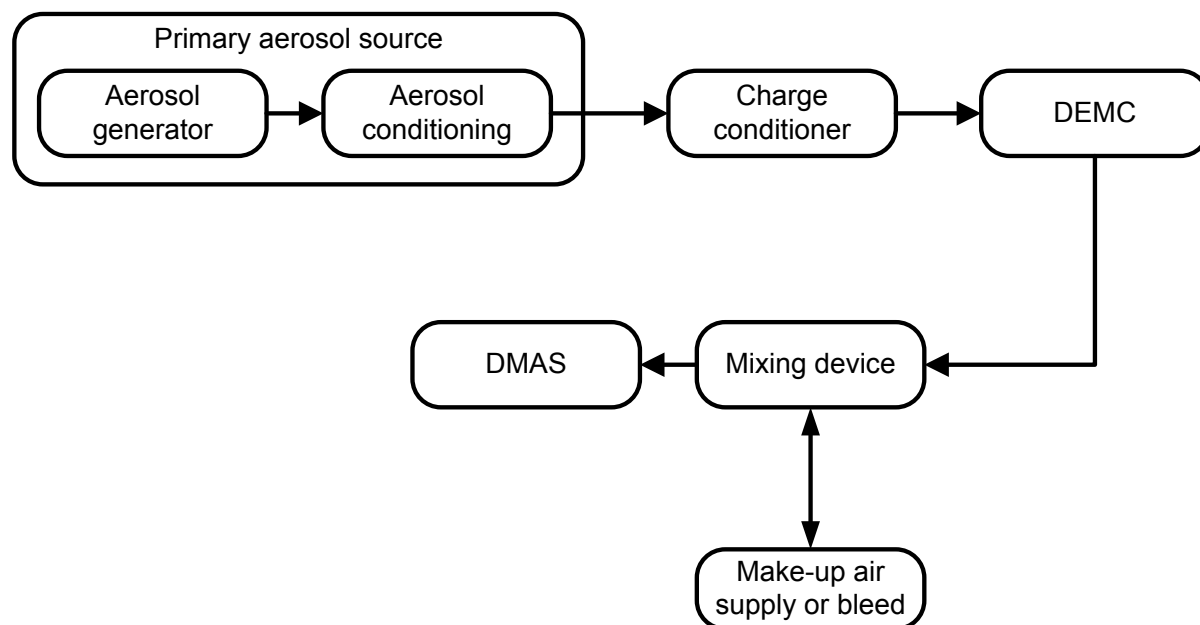
Figure E.2 — Setup for the measurement of the fraction of multiply charged particles with a DMAS.
