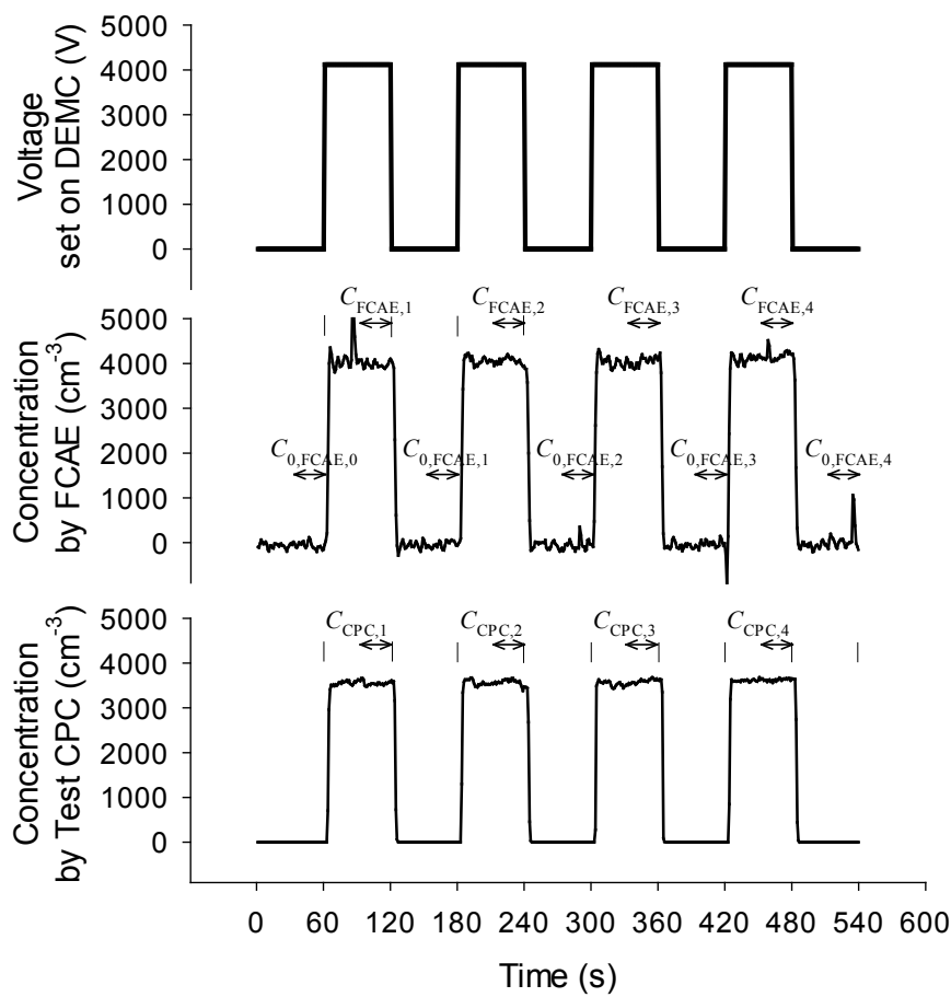
Figure M.1 — Example of DEMC voltage cycling and corresponding FCAE and test CPC concentration readings
