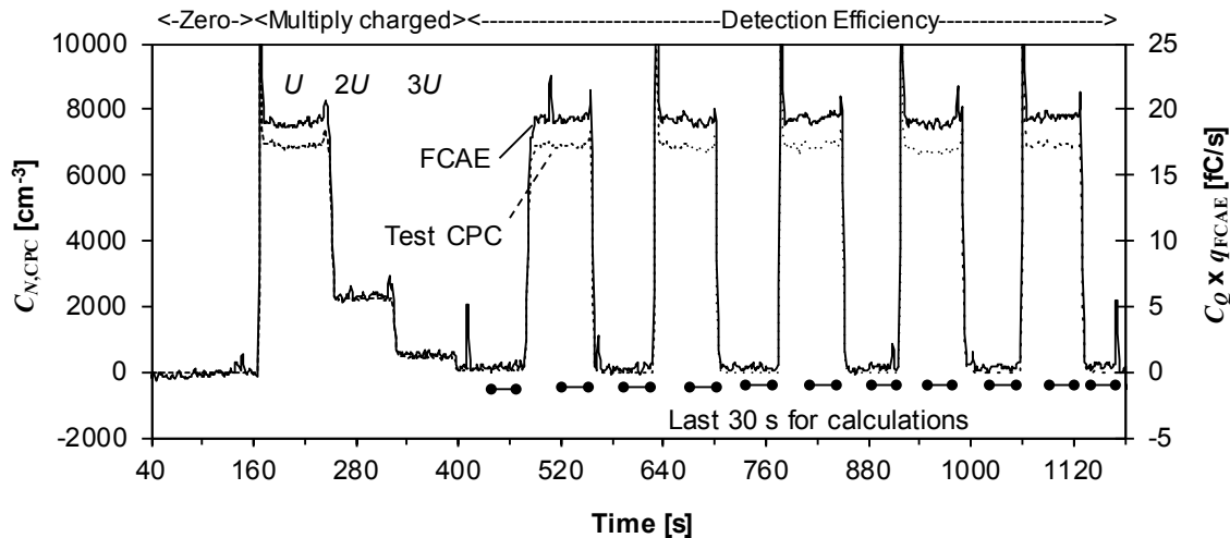
Figure J.3 — Example of calibration procedure of one detection efficiency
