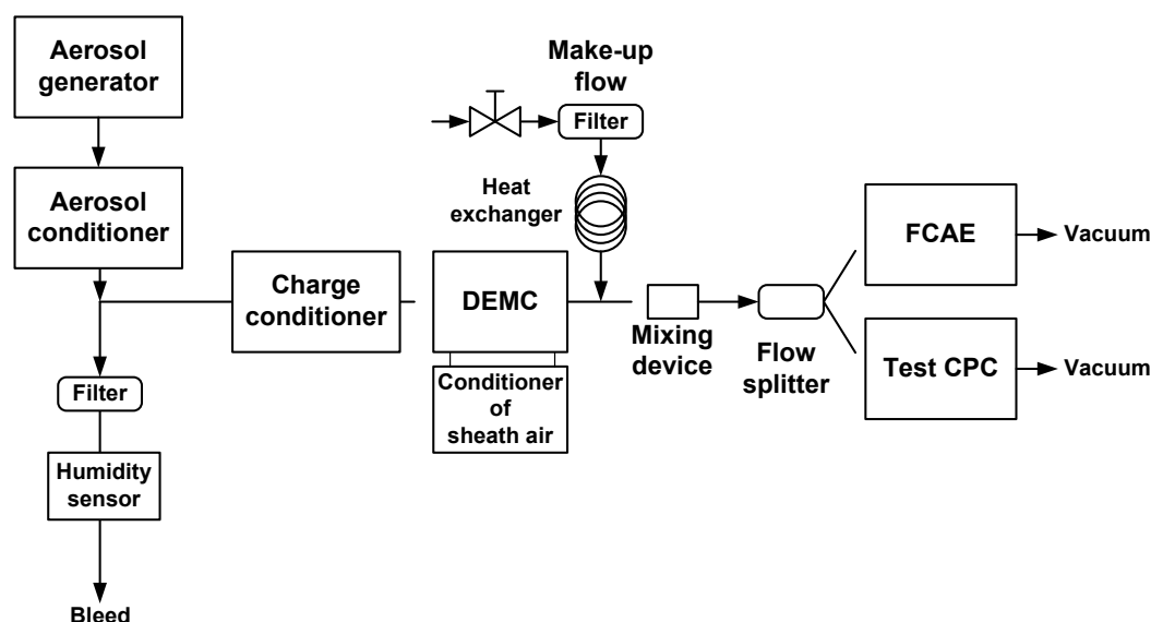
Figure J.1 — Experimental setup of the hypothetical example
