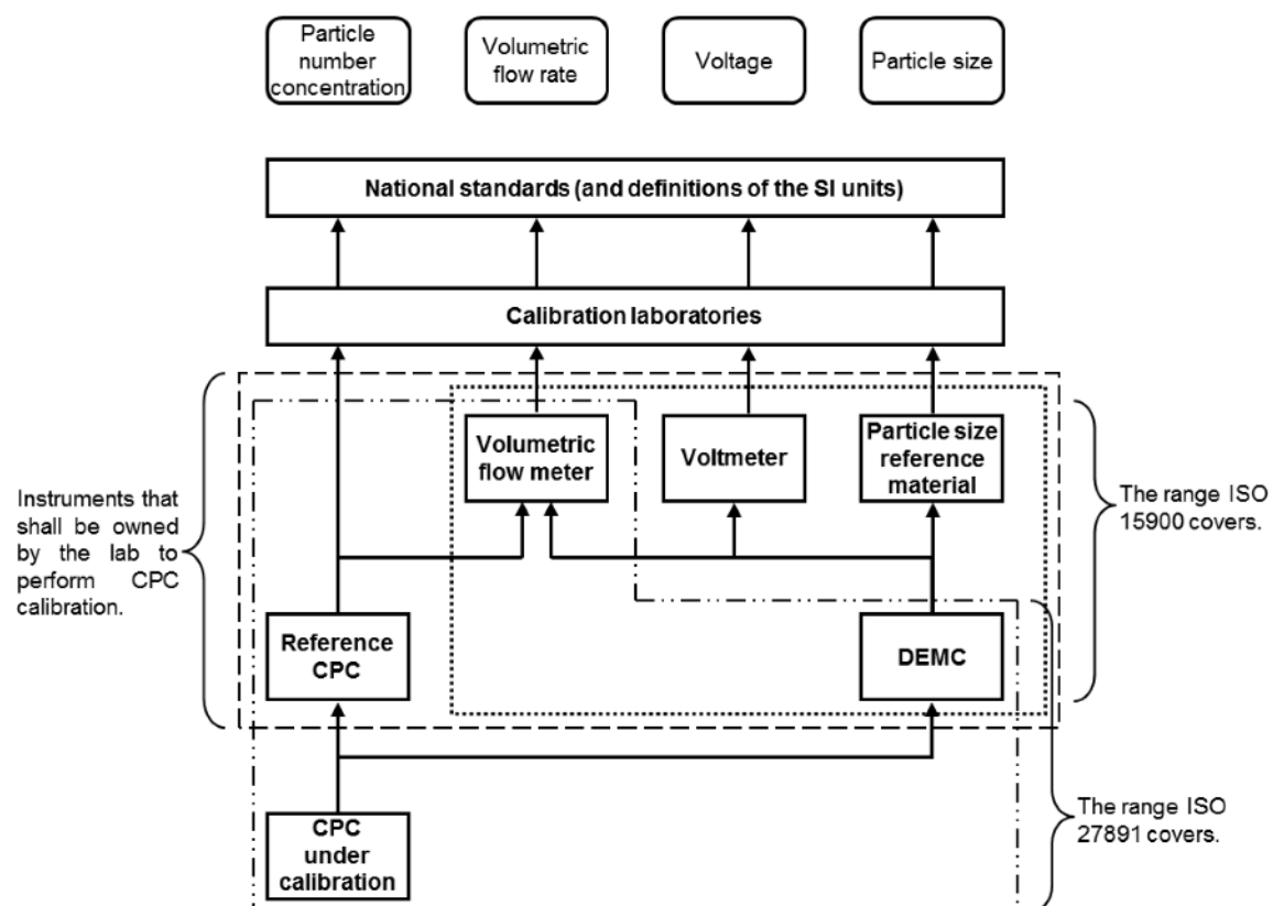
Figure F.2 — Traceability diagram for calibration with a reference CPC
