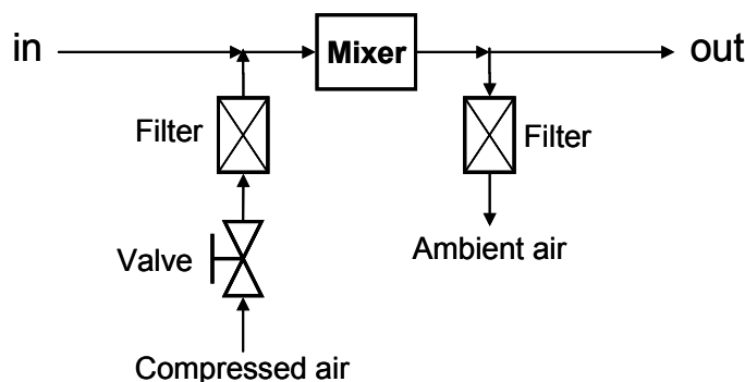
Figure G.3 — Schematic of the diluter with addition of clean air and bleeding of excess air
