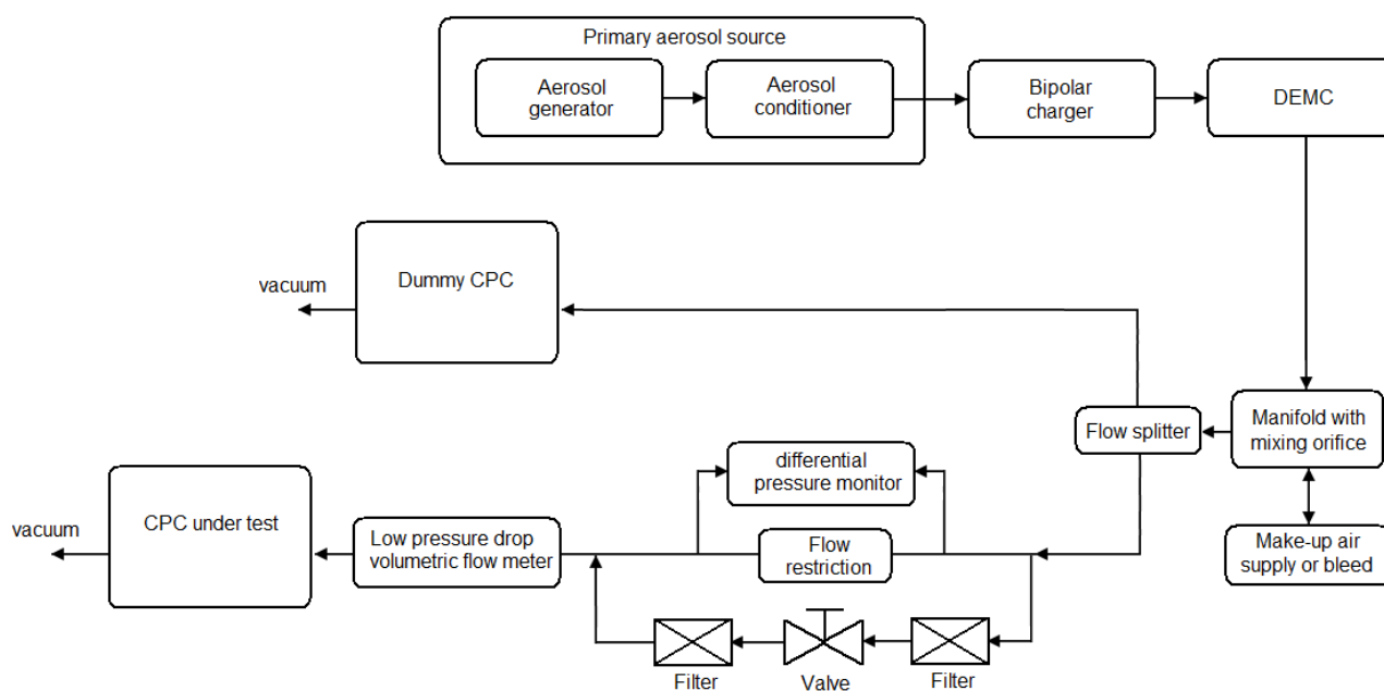
Figure I.2 — Schematic of the setup to validate the recommended diluter and CPC configuration
